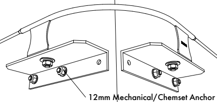
SL224.20 - Wall Mount Corner Module
